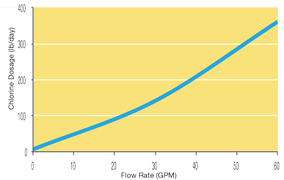
CHLORINATOR DELIVERY RATE MODEL 3150
